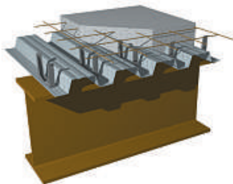
Non-welded connectors
