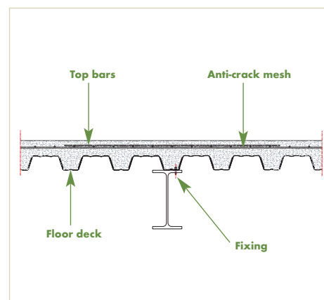
Beam parallel to the ribs
