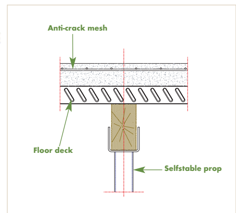
Standard section prop
