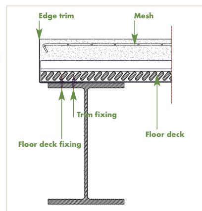
Trim fixed on steel support
