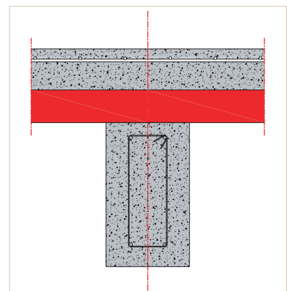
Continuous laying on concrete beam
