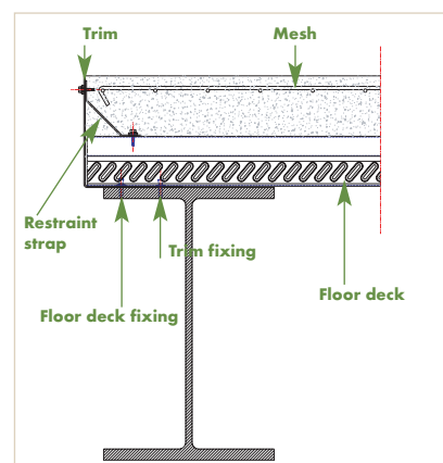
Trim fixed on steel support and restraint strap
