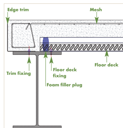
End support with embedded reinforcement on steel beam
