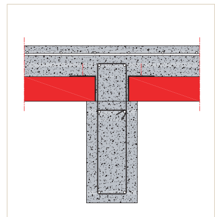
Laying with rebates on concrete beam
