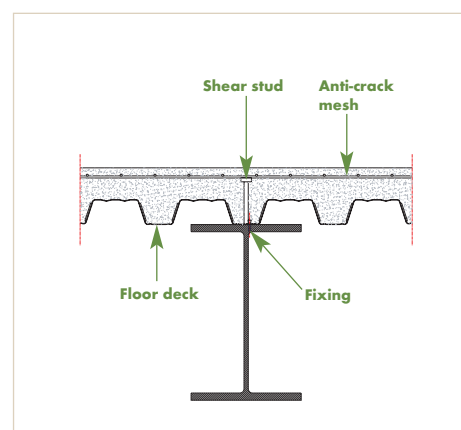
Composite beam
