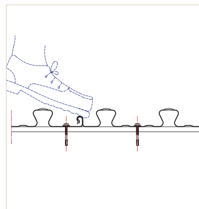
Cofrastra 40 interlocking
