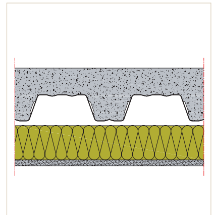
Thermal insulation over ceiling
