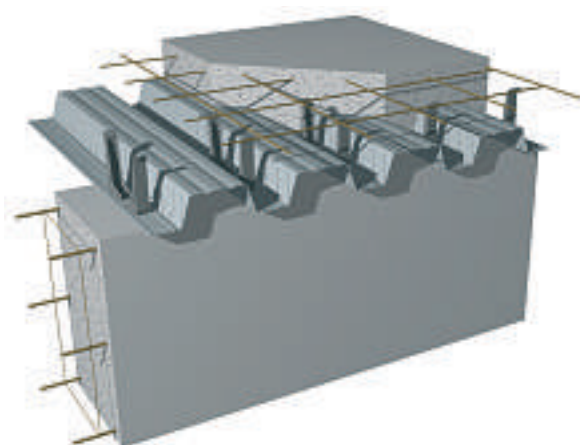
Continuous laying
