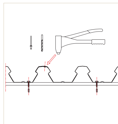
Cofrastra 70 interlocking
